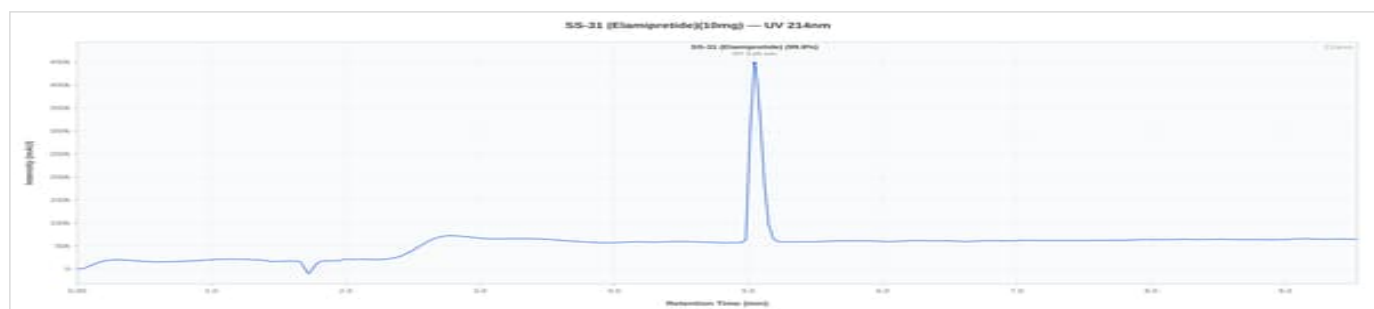
ss31 10mg - 08/26: UV Chromatogram
